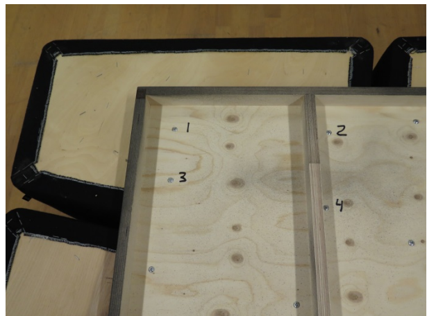
Figure 5 Elements attachment to base
